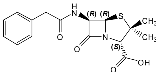
penicillin
