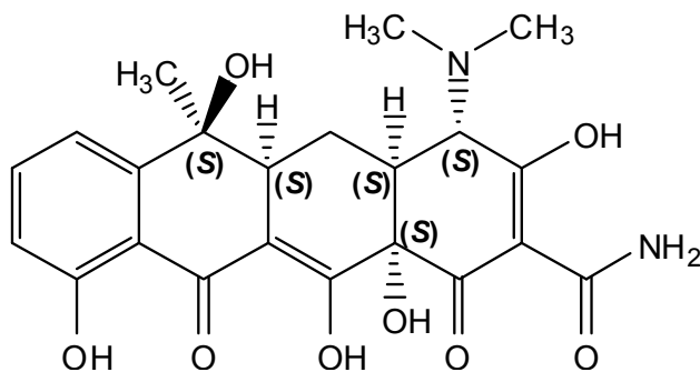
tetracycline
